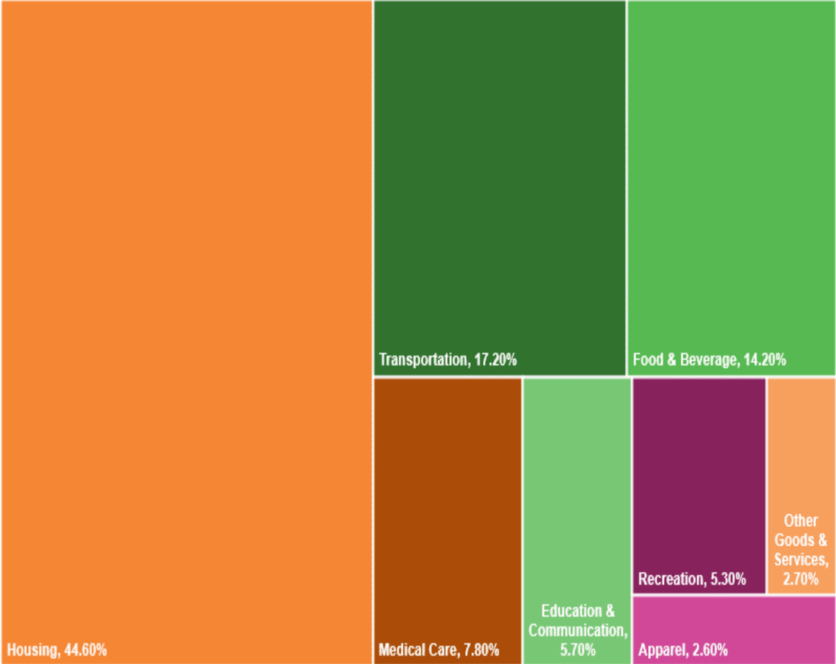
CPI Breakdown Sector Weighting
